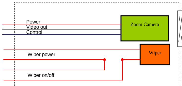
P15. SVEX-T300B inner structure, integrated camera installation
